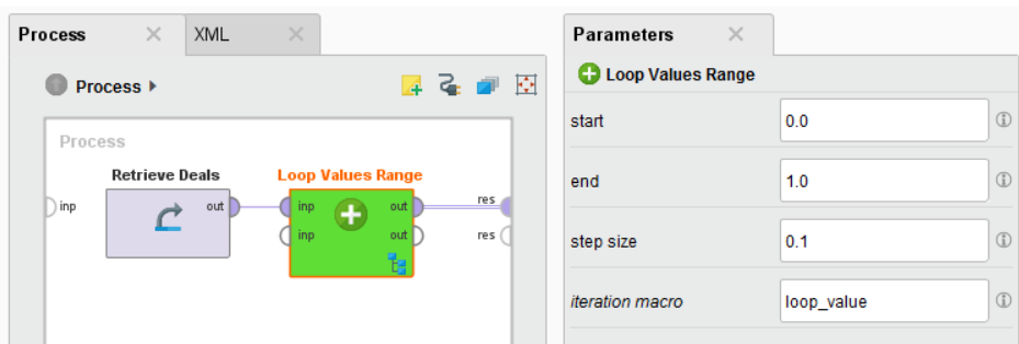
Figure 9.2: Super operator with parameters
