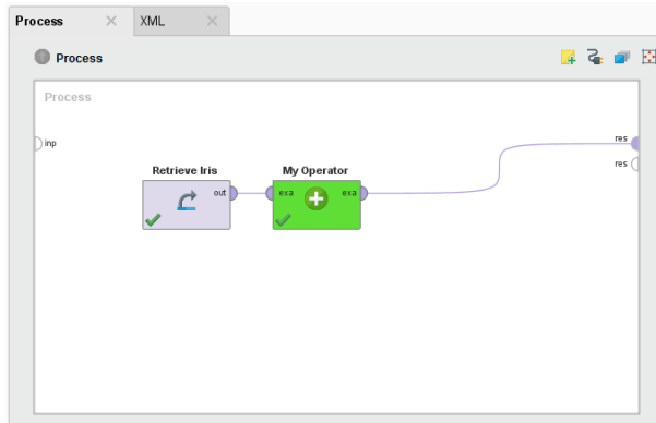
Figure 5.2: Operator with connected input and output ports
