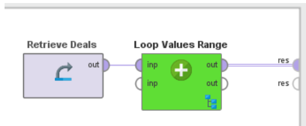
Figure 9.1: Super operator
